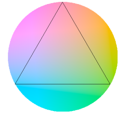
Figure 3: Cross section with constant L . For k = 3 , colors are mixed within the triangle.
